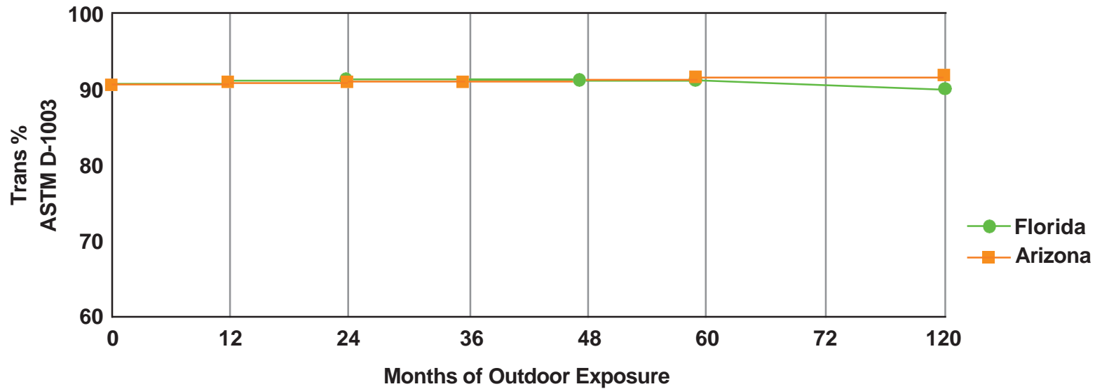
Luminous Transmittance During Outdoor Exposure Testing
