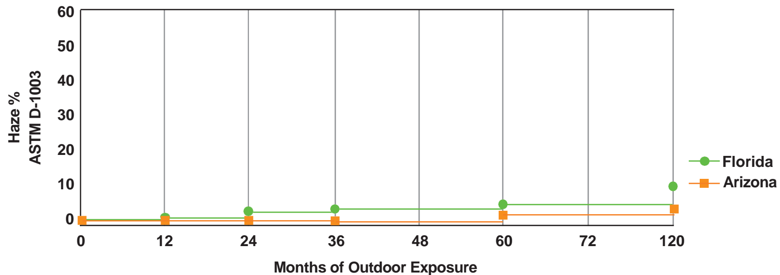
Optical Haze During Outdoor Exposure Testing
